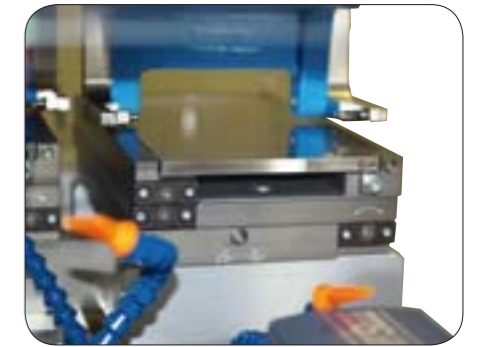
Cliché adjustment XYR by means of setscrew
